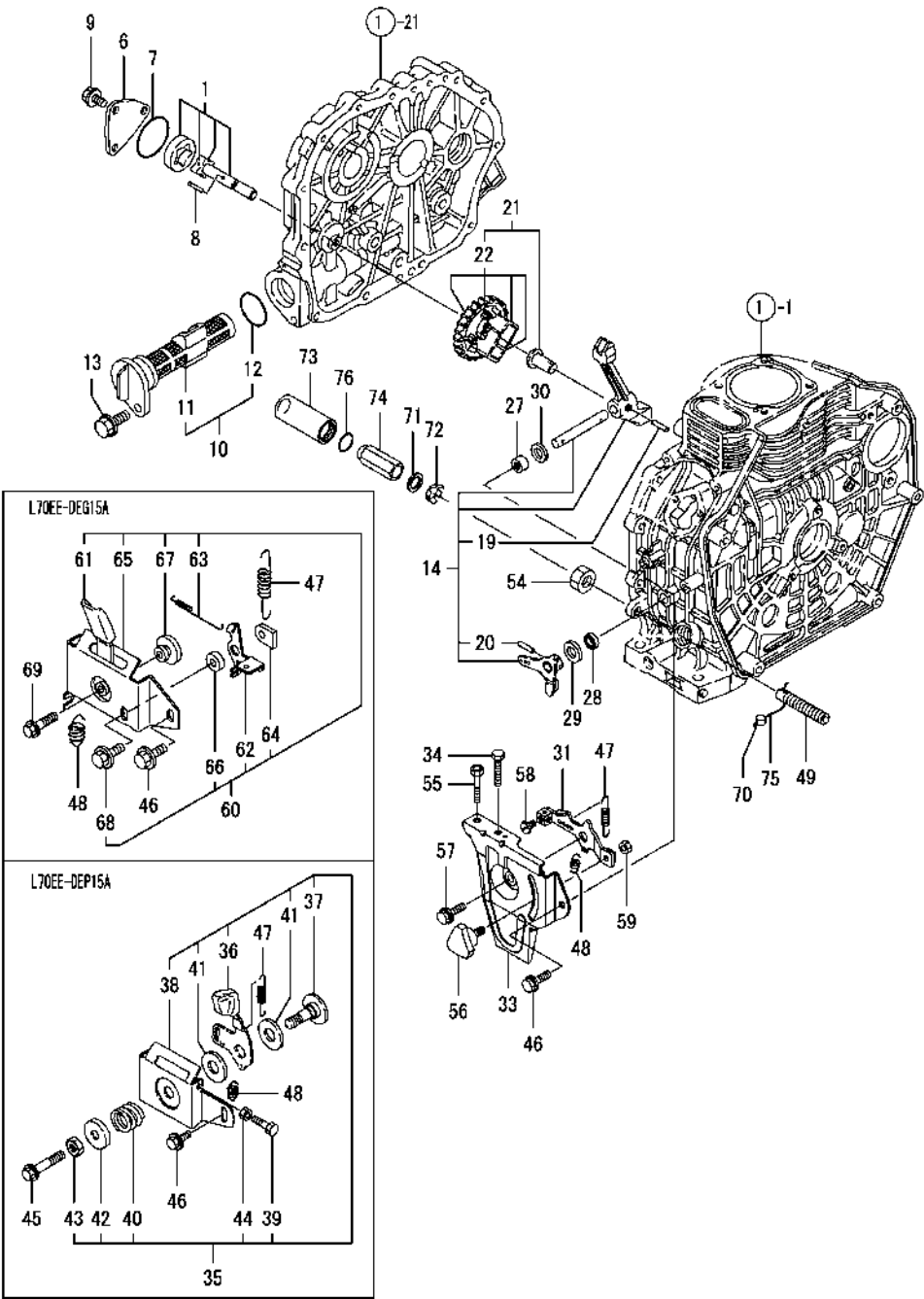
Fig.6. LUB.OIL PUMP & GOVERNOR
