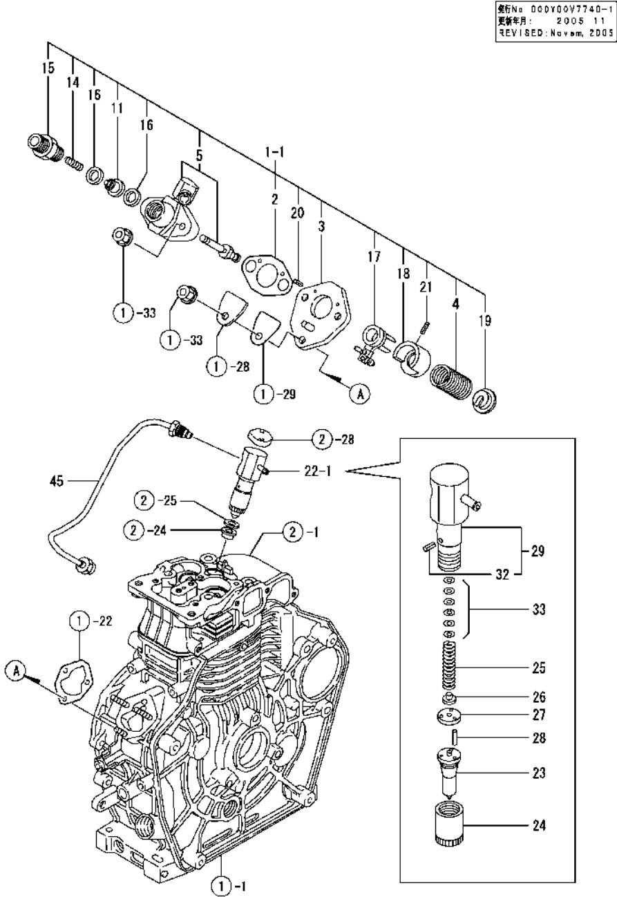
Fig.7. FUEL INJECTION PUMP
