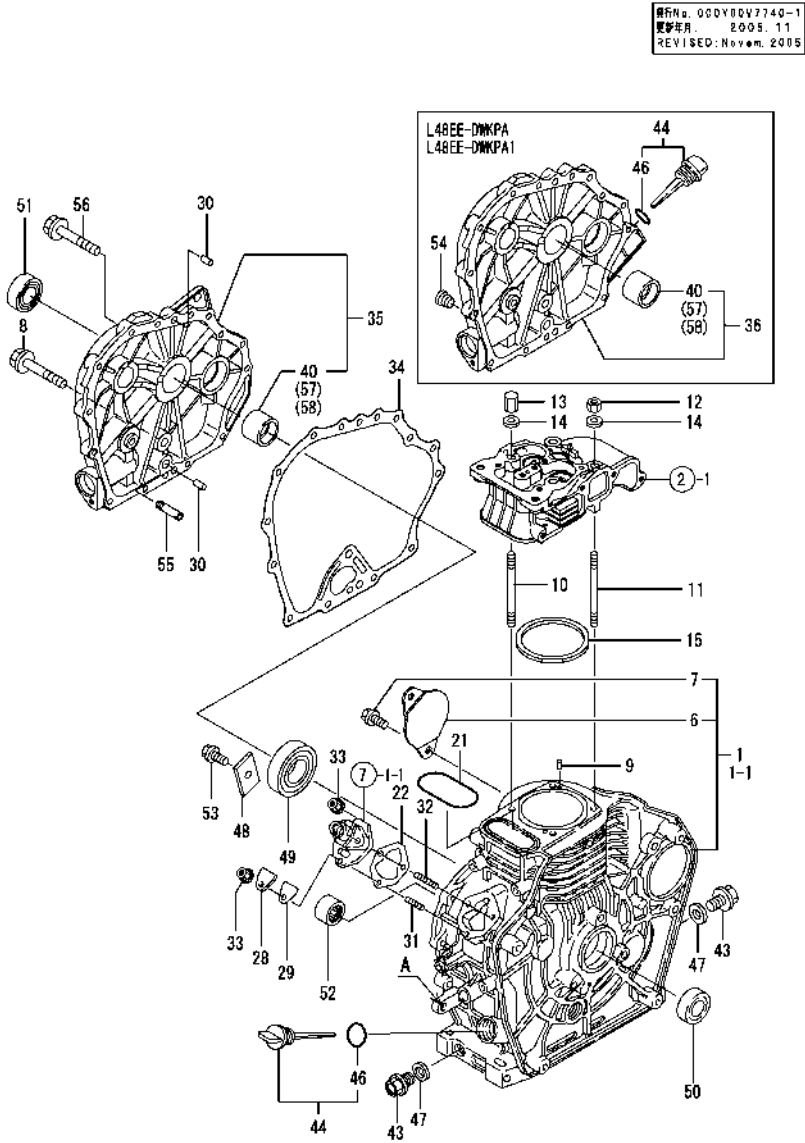
Fig.1. CYLINDER BLOCK
